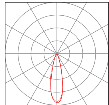
26° Lens — C0 / C180 cd / 1000 lm ..... C90 / C270
